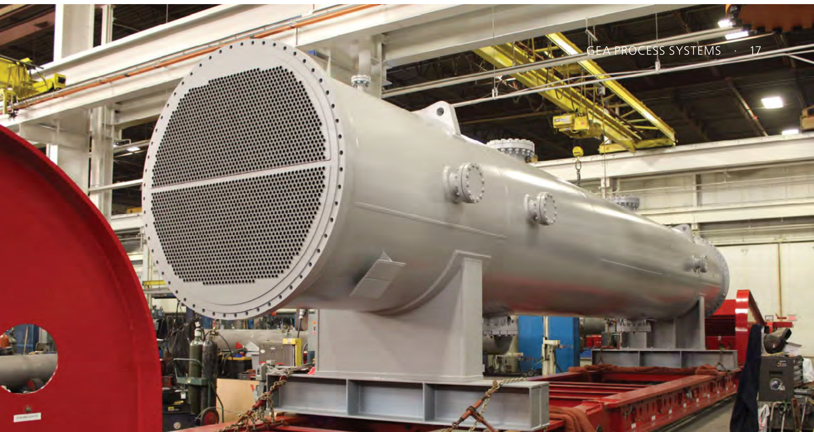
50" OD x 408" tube length propylene condenser
